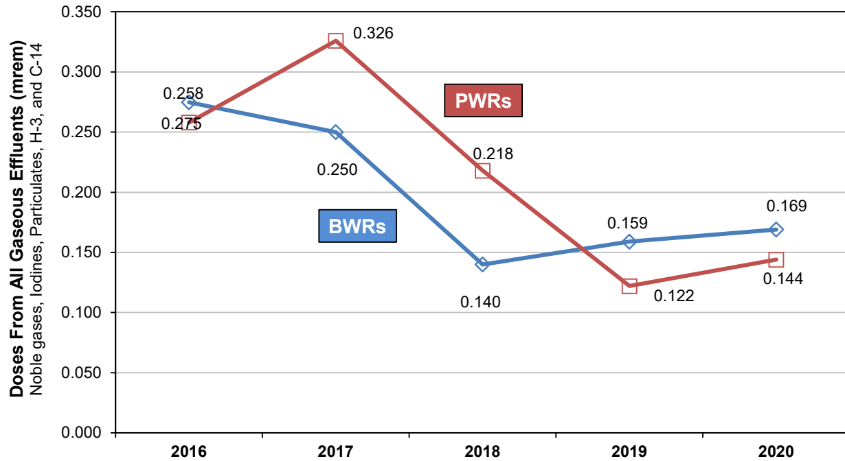
Figure 3-21 Median Maximum Annual Organ Dose, Gaseous Effluents 5-Year Trend, 2016–2020
