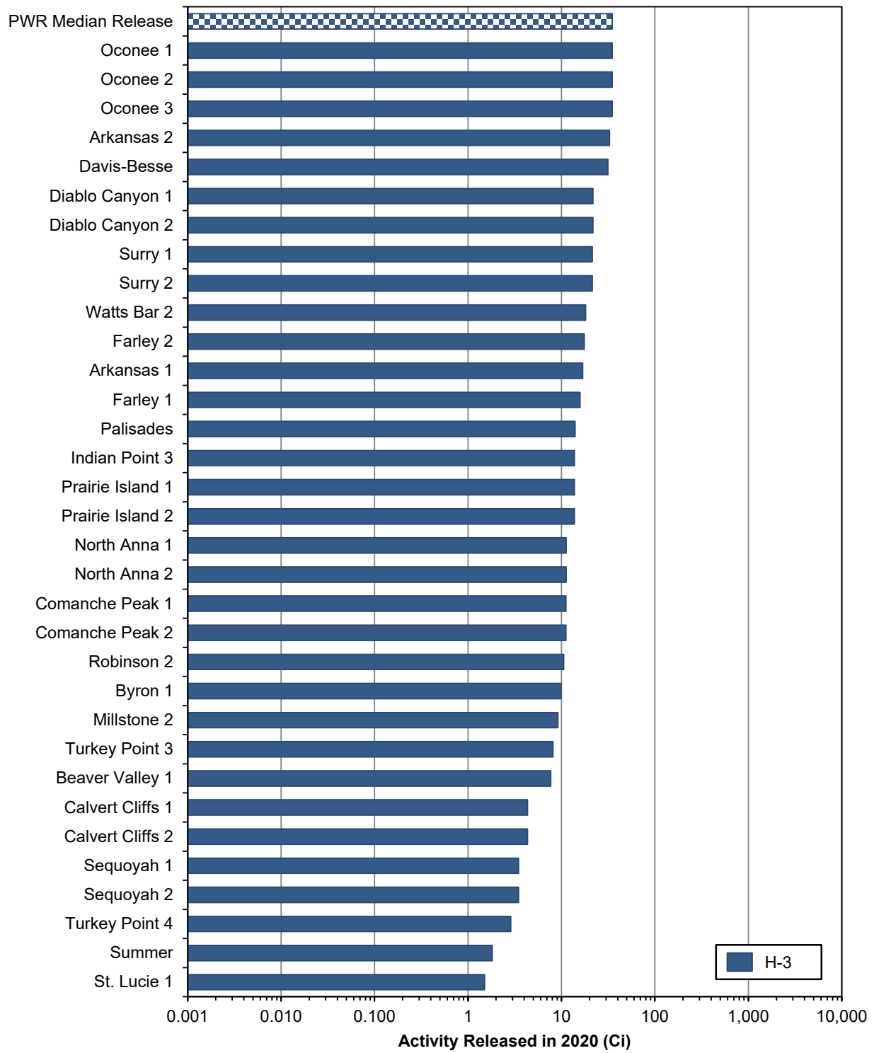
Figure 3-9 PWR Gaseous Releases — Tritium (continued)
