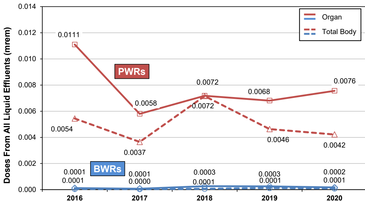
Figure 3-22 Median Maximum Annual Dose, Liquid Effluents 5-Year Trend, 2016–2020
