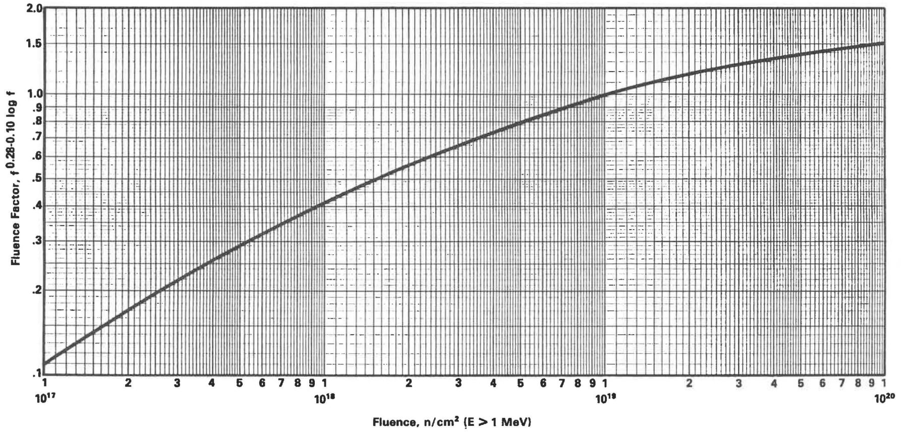
FIGURE 1 Fluence Factor for Use in Equation 2, the Expression for \Delta RT_{NDT}
